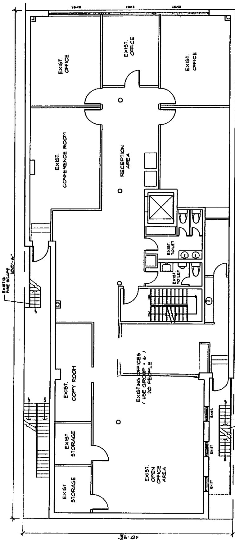
2ND FLOOR PLAN SCALE: 1/8" = 1'-0"
